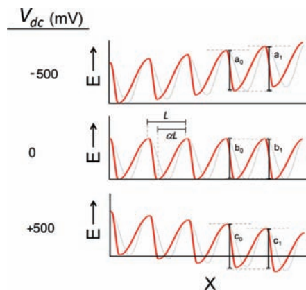
Figure 4. Schematic representation of the one-dimensional asymmetric periodic potential model ( \alpha = 0.7 ) in the presence of a +500 , 0 , and -500 mV dc bias, as labeled. The asymmetric periodic potential is shown by the solid line while a symmetric periodic potential is shown by the gray dashed line. a_0 and a_1 refer to the energy barrier height into the pore (toward the left) and out of the pore (toward the right) in the presence of a -500 mV dc bias, respectively. b_0/b_1 and c_0/c_1 have analogous meanings at 0 and 500 mV dc bias.
