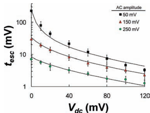
Figure 8. Mean escape time for HP-A 50 to escape from the \alpha HL pore, as a function of applied DC bias at three different AC amplitudes (50 mV, 150 mV, 250 mV) and at a temperature of 0 °C. The solid lines correspond to best fits, using the one-dimensional asymmetric periodic potential model described by eq 5.
